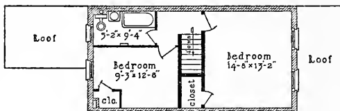
Second-floor Plan
